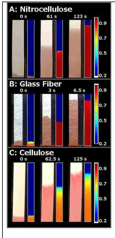
Figure 28: Experimental and modeled 4 cm wetting in various membranes. A: HF135 nitrocellulose. B: 8964 glass fiber. C: CFSP223 cellulose.
