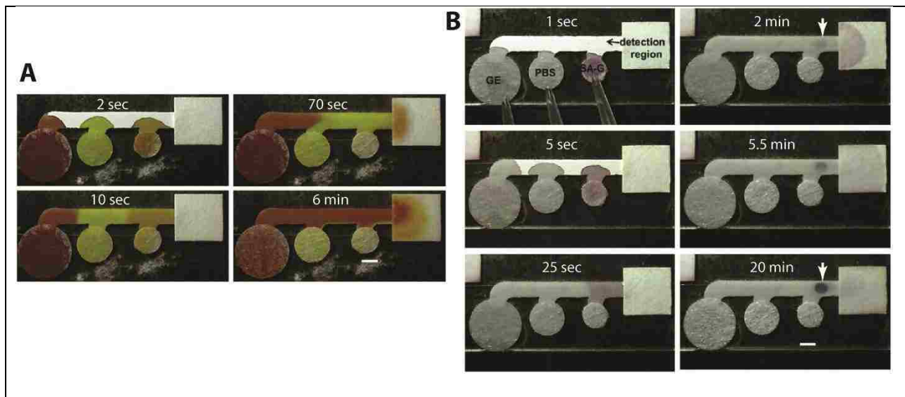
Figure 120: A 2DPN designed to automate a multi-step signal amplification [figure source: Fu, Kauffman, Lutz, Yager, “Chemical signal amplification in two-dimensional paper networks,” Sensors & Actuators B 149 (2010) 325–328]. Porous (glass fiber) pads were used to hold finite volumes of source fluids. A) Image sequence of delivery of three fluids to a common leg in a timed sequence (orange, yellow, red). B) Image sequence for a sandwich immunoassay using a multi-step signal amplification process (SA-G: streptavidin-gold; PBS: phosphate-buffered saline; GE: gold enhancement reagent). The upper right image shows a faint gold spot (end point of a typical LFT), and the lower right image shows the darkened spot after enhancement. The device carried out all delivery steps without intervention. The width of the main channel was 3 mm.
