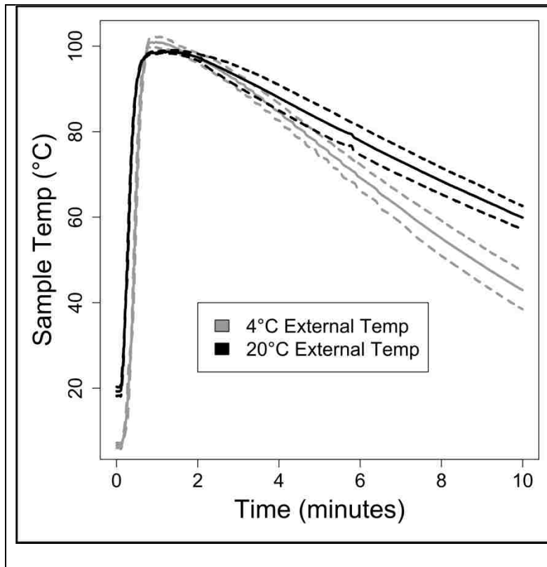
Figure 59: Chemical heater performance in varied ambient conditions. The chemical heater was run either in laboratory conditions (20°C) or in a cold room (4°C). The chemical heater was designed with enough MgFe fuel and NaCl to perform well even in cold ambient conditions. Solid lines are means, dotted lines are \pm one standard deviation, n=3 .
