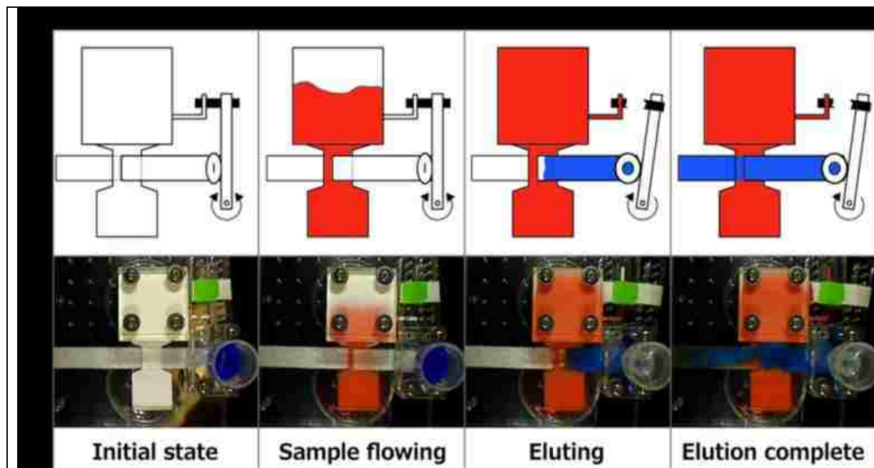
Figure 66. Automating the p-switch for the large volume sample concentration. Initially, the elution buffer well is full, but the tubing connecting the well to the secondary network is pinched closed. Once the sample (red) is added, it flows through the primary network into the waste pad. When the waste pad reaches a sufficient level of saturation, the activation leg wets a water-soluble paper, weakening it and causing the arm to release the pinch on the elution tube. When the pinch is relieved, the elution buffer (blue) flows through the junction and fills the secondary network.
