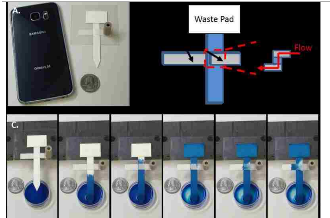
Figure 63: Demonstration of p-switch operation. A. Image of a simple p-switch device with a Galaxy S6 mobile phone and US quarter for scale. B. Schematic of p-switch device consisting of multiple materials and a cross-section of the junction. C. Images from a video showing fluid flow in a p-switch device.
