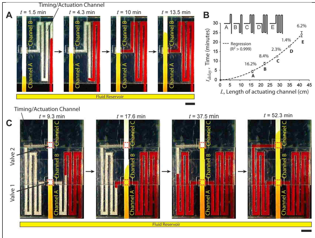
Figure 98: Programming valve actuation time. A. Time-lapse images of an on-switch with a serpentine actuation channel that times valve actuation. Channel A and the actuation channel were connected to a common fluid reservoir. Yellow fluid was added in the reservoir at time, t = 0 . The fluid reached the end of channel A at 4.3 min. Fluid in the timing/actuation channel reached the actuator at 10 minutes and actuated the valve. Note that the fluid appears darker in the actuation channel because it is thicker than channels A and B. B. Time required for fluid to traverse the length of different lengths of serpentine glass fiber channels. Percent values are coefficients of variation ( N = 6 ). C. Time-lapse images of a device consisting of two on-switches (valve 1 and valve 2; dotted red squares) that actuate sequentially by a common timing/actuation channel. Valves actuated when fluid in the timing channel reached the corresponding actuators.
